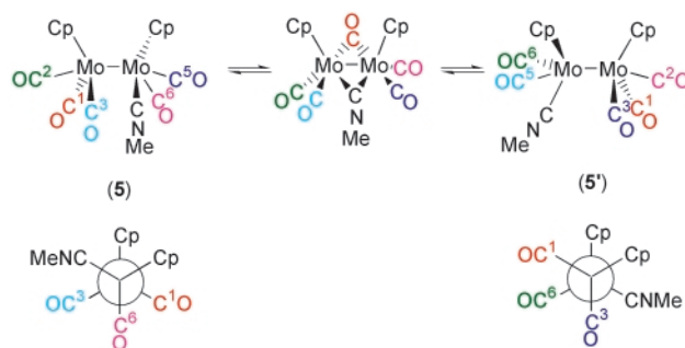
Scheme 3 The mechanism of carbonyl and methyl isocyanide exchange between the molybdenum atoms in cis -[( \eta^5 -C 5 H 5 ) 2 Mo 2 (CO) 5 (CNMe)], (5). Colours are used to identify the carbonyls during the exchanges. Hence the exchange path followed by carbonyl, 5–2(green), can be identified by looking for the green carbonyl in each structure. (Note the bold 5 refers to structure (5) and the 2(green) to C 2 O(green).) Comparison with Fig. 1 shows that this produces the pairwise carbonyl exchanges 5–2(green) \rightleftharpoons 5'–6(green)/5–6(magenta) \rightleftharpoons 5–2(magenta); 5–3(blue) \rightleftharpoons 5'–5(blue)/5–5(purple) \rightleftharpoons 5'–3(purple); and 5–1(red) is unaffected. The cyclopentadienyl groups also exchange.
