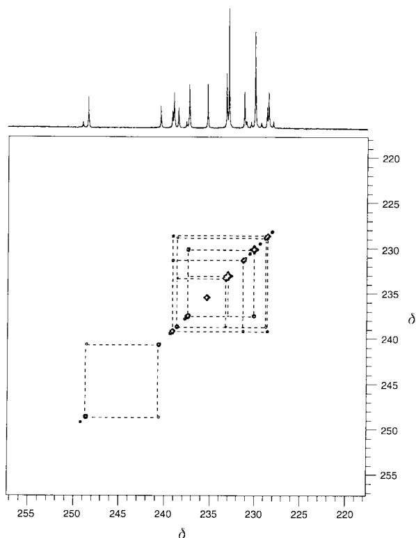
Fig. 4 The COSY-90 100.62 MHz ^{13}\text{C} NMR spectrum of ^{13}\text{CO} -enriched [(\eta^5\text{-C}_5\text{H}_5)_2\text{Mo}_2(\text{CO})_5(\text{CNMe})] in (\text{CD}_3)_2\text{NCDO} at -62^\circ\text{C} .
