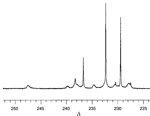
Fig. 5 The 100.62 MHz ^{13}\text{C} NMR spectrum of ^{13}\text{CO} -enriched [(\eta^5\text{-C}_5\text{H}_5)_2\text{Mo}_2(\text{CO})_5(\text{CNMe})] in (\text{CD}_3)_2\text{NCDO} at -13^\circ\text{C} .
