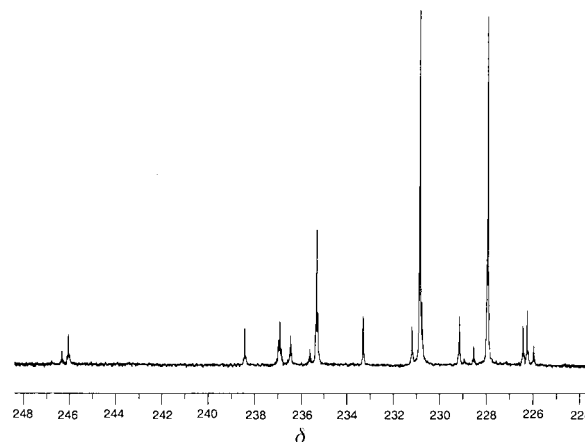
Fig. 6 The 100.62 MHz ^{13}\text{C} NMR spectrum of ^{13}\text{CO} -enriched [(\eta^5\text{-C}_5\text{H}_5)_2\text{Mo}_2(\text{CO})_5(\text{CNMe})] in (\text{CD}_3)_2\text{CO} at -70^\circ\text{C} .
