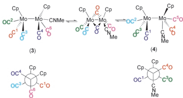
Scheme 2 The mechanism of carbonyl and methyl isocyanide exchange between the molybdenum atoms in gauche,cis -[( \eta^5 -C 5 H 5 ) 2 Mo 2 (CO) 5 (CNMe)], (3) and (4). Colours are used to identify the carbonyls during the exchanges. Hence the exchange path followed by carbonyl, 3–1(red), can be identified by looking for the red carbonyl in each structure. (Note the bold 3 refers to structure (3) and the 1(red) to C 1 O(red).) The numbering follows that in Fig. 1. The exchange produces the pairwise carbonyl exchanges 3–1(red) \rightleftharpoons 4–4(red); 3–2(green) \rightleftharpoons 4–3(green); 3–3(blue) \rightleftharpoons 4–2(blue); 3–4(purple) \rightleftharpoons 4–1(purple); and 3–6(magenta) \rightleftharpoons 4–5(magenta).
